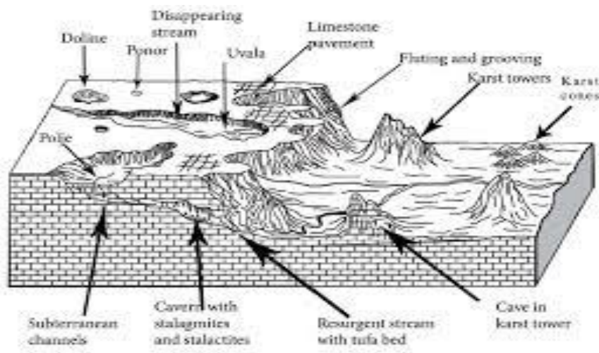
Figure 4.20: Karst features
